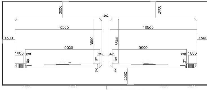
Typical Cross-Section of Cut And Cover Box For Maximum 30m Soil Cover
