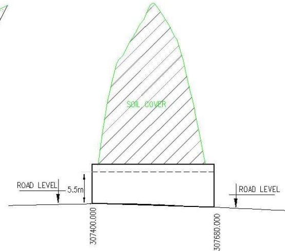
Typical Longitudinal section
