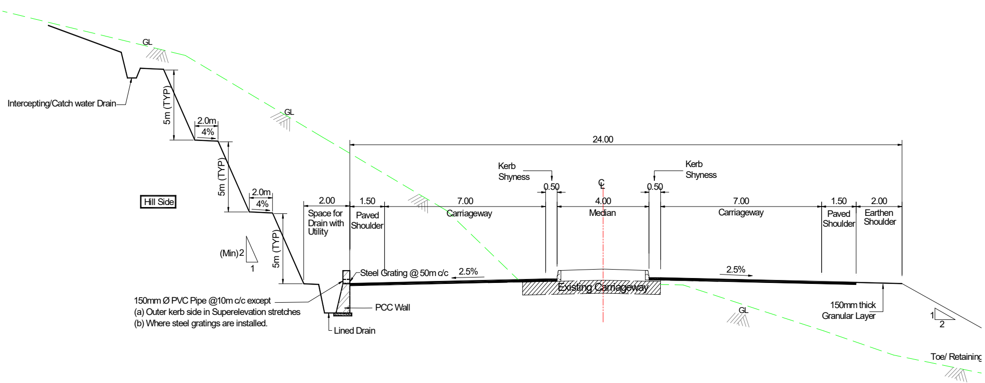
TCS-5 : 4-Lane Divided Carriageway (One Side Hill Cutting and Other Side Toe/Retaining Wall)
