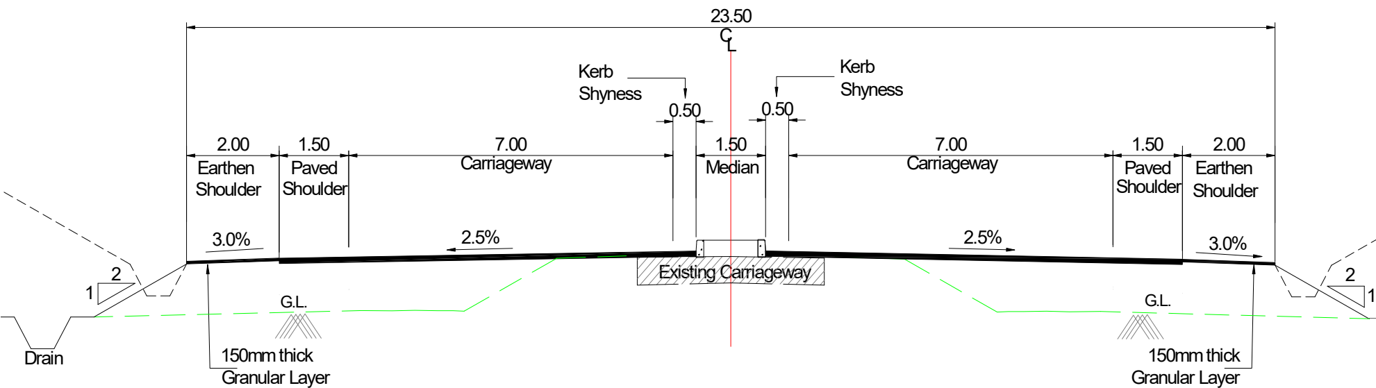
TCS-9 : 4-Lane Divided Carriageway With Cut/Fill (Semi Built up Area)
