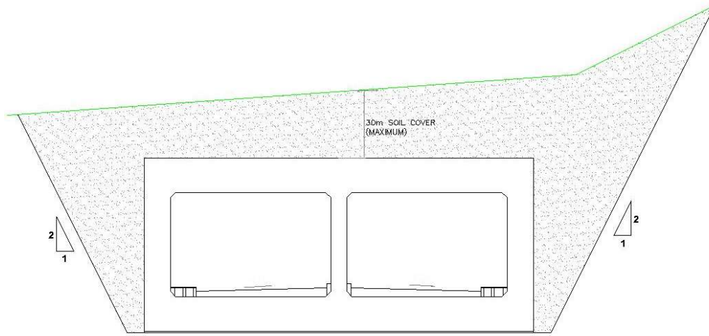
Typical Cross-Section
