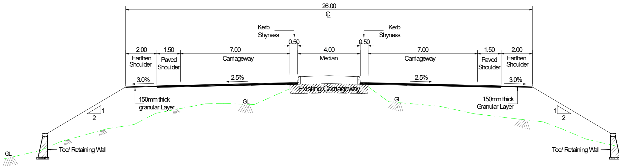
TCS-7 : 4-Lane Divided Carriageway with Bothside Toe/Retaining Walls
