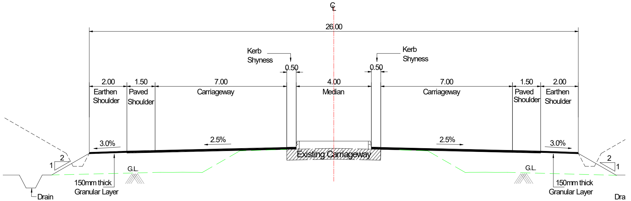
TCS-1 : 4-Lane Divided Carriageway With Raised Media (Normal Fill/Cut Section– Rural Section)
